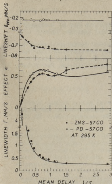
Fig. 4. Time-dependences of central line parameters for ^{57}\text{Co} in Pd and ZnS— ^{57}\text{Co} \gamma -sources. The dashed line for \delta(T) is an empirical dependence \delta(t) = [-0.74 + 0.14 \exp(-t/40)] mm/s ( t in ns) to fit the data. The solid lines for \epsilon(T) and \Gamma(T) are the corresponding theoretical dependences calculated for \beta=8 , according to [8].
