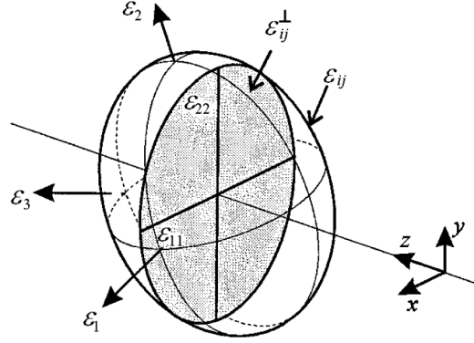
Fig. 3. The polarization of light is influenced by the components of the dielectric tensor which lie in the xy plane, perpendicular to the wave normal z .
