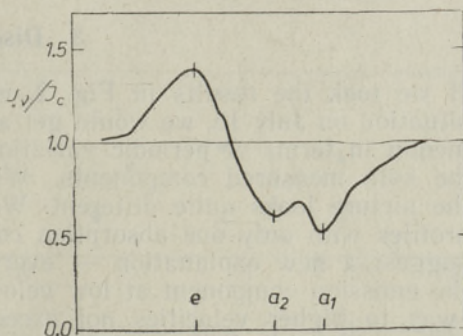
Fig. 1. Typical profile of a higher member of the Balmer series. The positions of different line components are marked.
