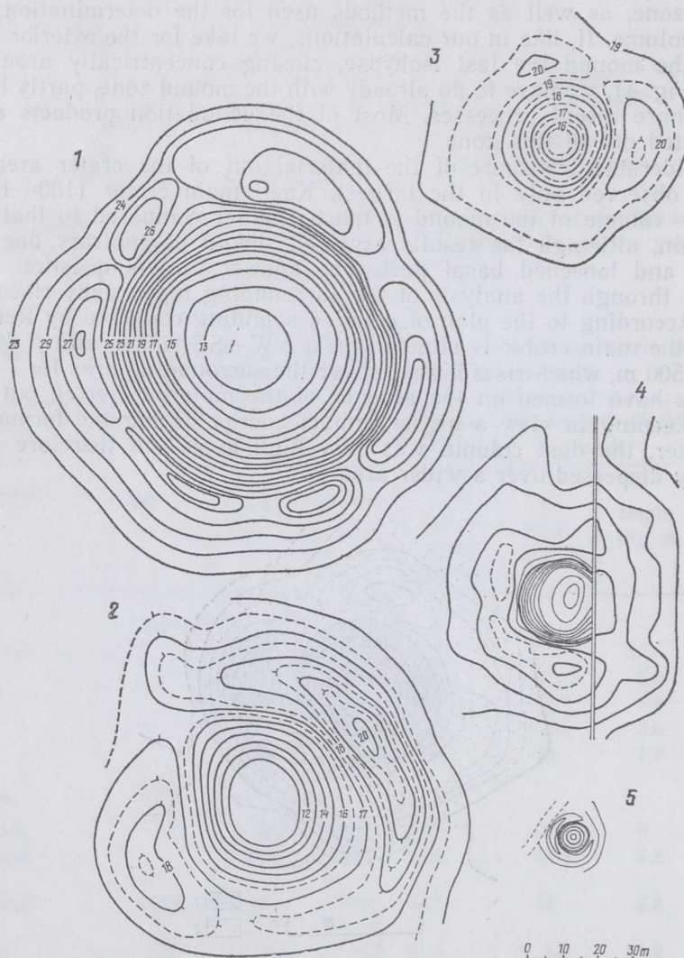
Fig. 5. Morphologically better preserved meteorite craters of Estonia (in comparable measure). 1, Kaali main crater (100 m); 2, Ilumetsa Põrguhaud (76 m); 3, Ilumetsa Süvahaud (47 m); 4, Tsõõrikmägi (40 m); 5, Simuna (9 m).
