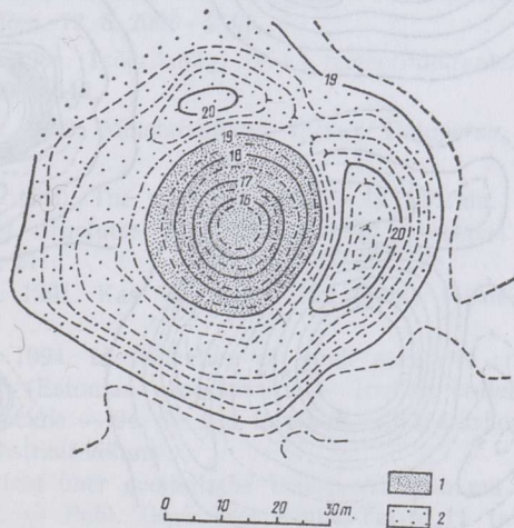
Fig. 4. Ilumetsa Süvahaud. An example of determining the mound volume basing on a detailed topographical plan. Close hatching shows the depression, sparse hatching marks the mound area. The boundary coincides with the last, 19 m isohypse, closing concentrically around the mound.
