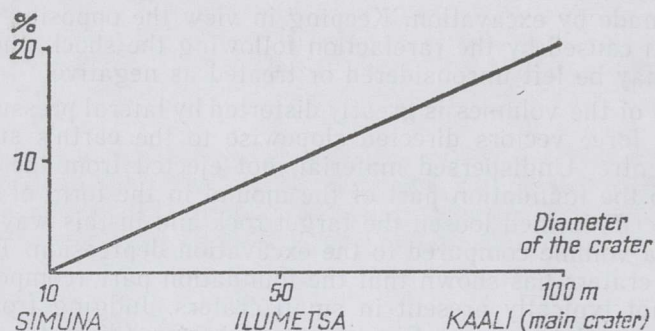
Fig. 3. Supposed increase of the mound volume on the account of the lifted basal part depending on the diameter of the crater (in per cent with respect to the volume of the crater depression).
