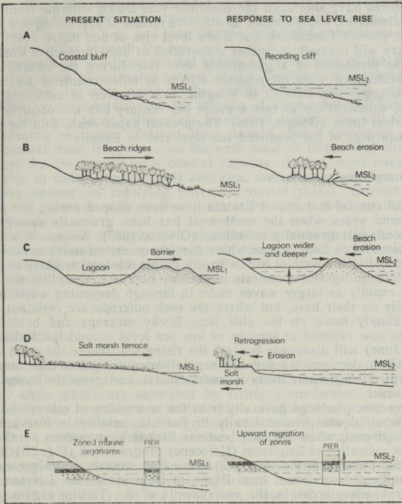
Fig. 2. Present situation of coastal features in Estonia, and probable responses to a sea level rise in the Baltic.
