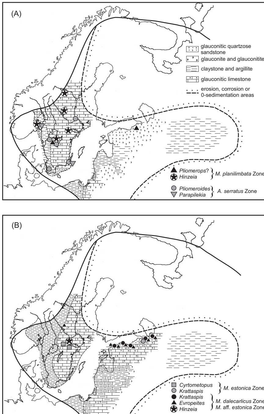
Fig. 3. Facies distribution of the Baltoscandian palaeobasin (modified after Erdtmann 1965; Männil 1966; Laškovas 1968; Modlinski 1976; Erdtmann & Paalits 1994) showing cheirurin data: (A) during the Hunneberg, for comparison the Tremadoc cheirurins from the A. serratus Biozone are shown (grey filling); (B) during the Billingen (Pärnaste 2004b).
