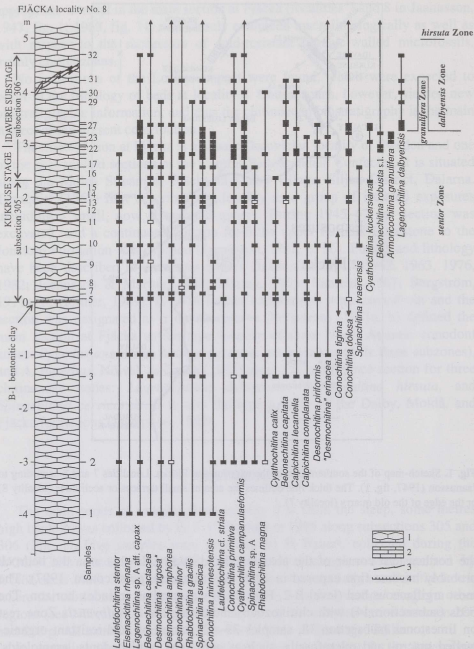
Fig. 2. Faunal log showing the range of chitinozoans in the upper part of the Dalby Limestone (Upper Member in Jaanusson, 1982, p. 38) at Fjäcka locality 8. 1, semimodular limestone (parallel lines mark clayey intercalations); 2, bedded limestone; 3, fault; 4, K-bentonite bed. Open squares represent forms referred to as cf. The lower boundary of the hirsuta Zone, about 5 m above the bentonitic clay layer, is shown according to the data from sample 60-166 in Laufeld (1967).
