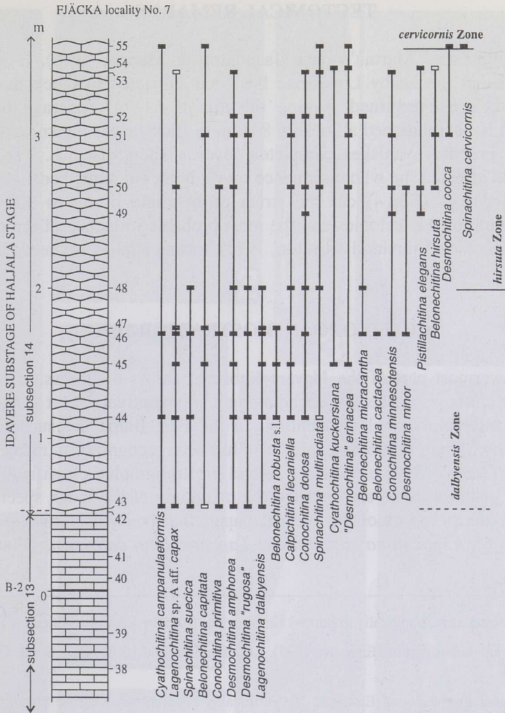
Fig. 3. Faunal log showing the range of chitinozoans in the middle part of the Dalby Limestone at Fjäcka locality 7. Barren samples 33–37 (see Fig. 1) are not shown. The dashed line marks the appearance level of chitinozoan fauna. For legend refer to Fig. 2.
