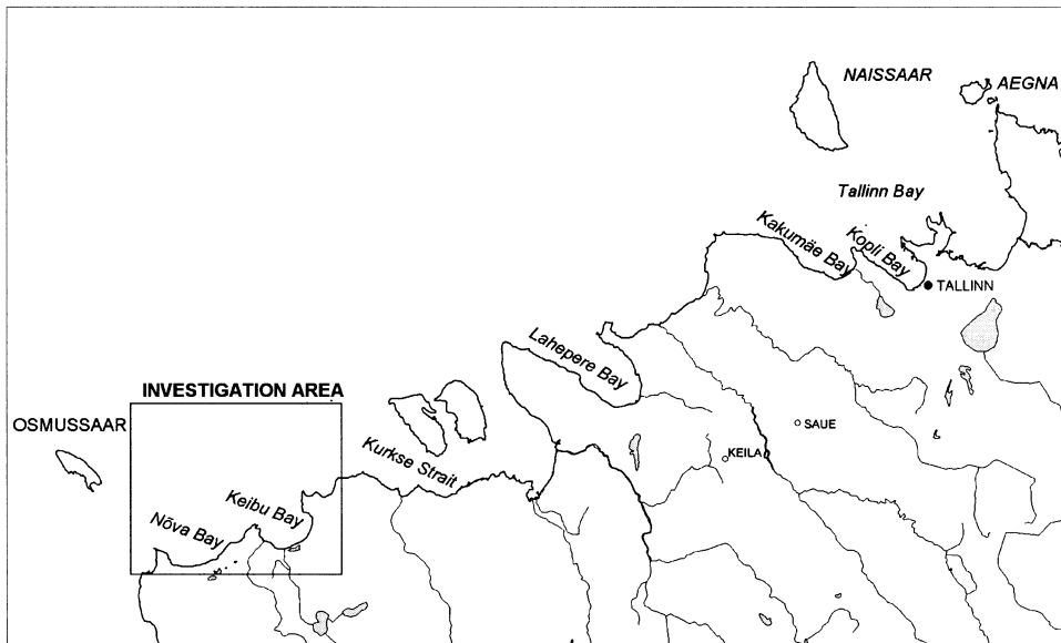
Fig. 1. Location of the investigation area.
