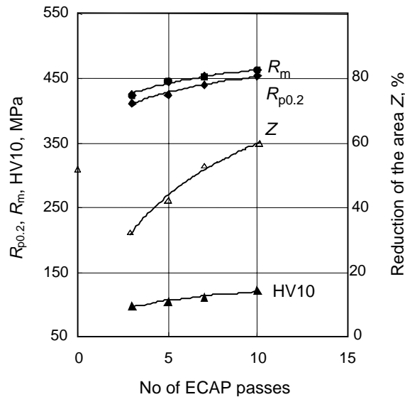
Fig. 3. Dependence of the strength and plastic properties of copper on the plastic deformation by ECAP.
