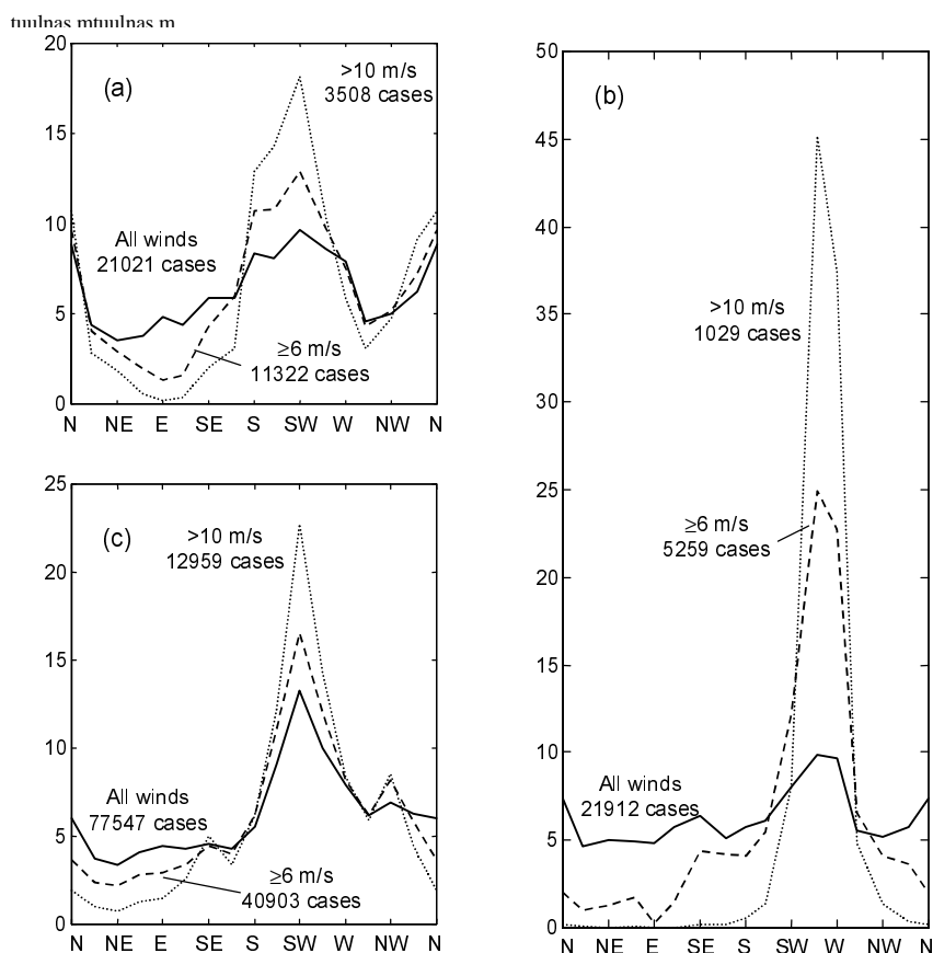
Fig. 3. Directional distribution of all winds (solid line), wind events with wind speed \geq 6 m/s (dashed line), and strong winds (> 10 m/s) (dotted line): (a) Vilsandi 1977–1991; (b) Ristna 1977–1991; (c) Näsudden 1980–1988, at 38 m level. Vertical axis represents relative frequency of occurrence of wind events, %.
