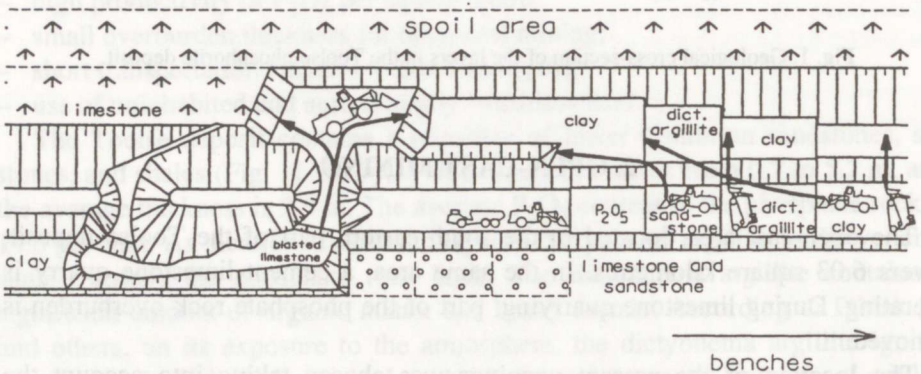
Fig. 3. Limestone stripping by dumping.
