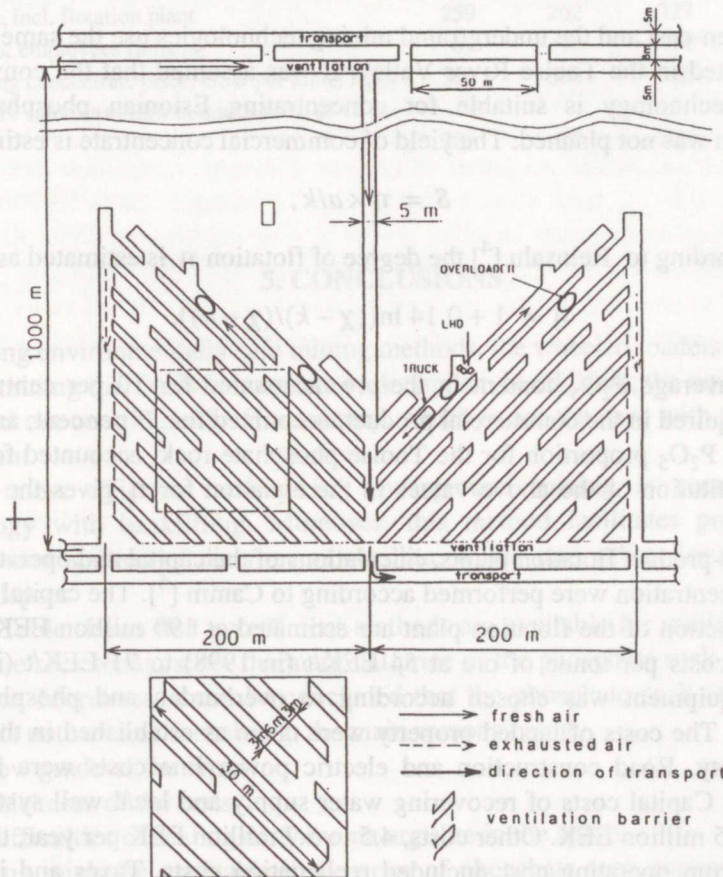
Fig. 5. Room-and-pillar mining.
