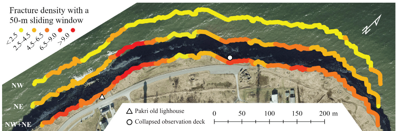
Fig. 8. Fracture density in Middle Ordovician carbonates within a 50-m sliding window, with separate profiles for NW-oriented, NE-oriented, and all joint sets.
