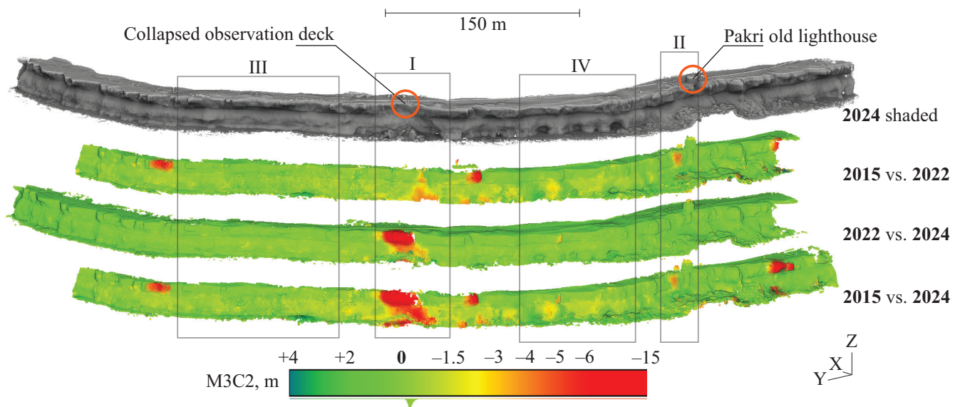
Fig. 11. Changes in a section of the cliff face over time. I – location of the collapsed observation deck, II – collapse of the limestone block, III – retreat of glauconitic sandstone, IV – notches. Abbreviation: M3C2 – model-to-model cloud comparison.
