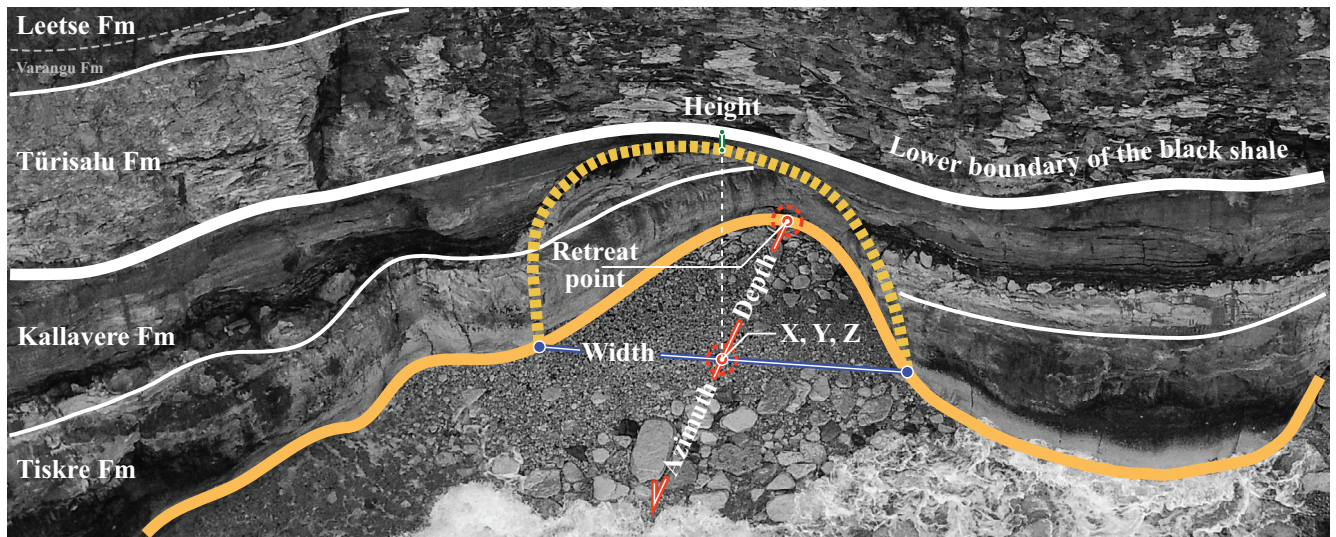
Fig. 6. Visualisation of the measured morphometric parameters of a coastal notch. The X, Y, and Z coordinates represent the midpoint of the notch mouth.
