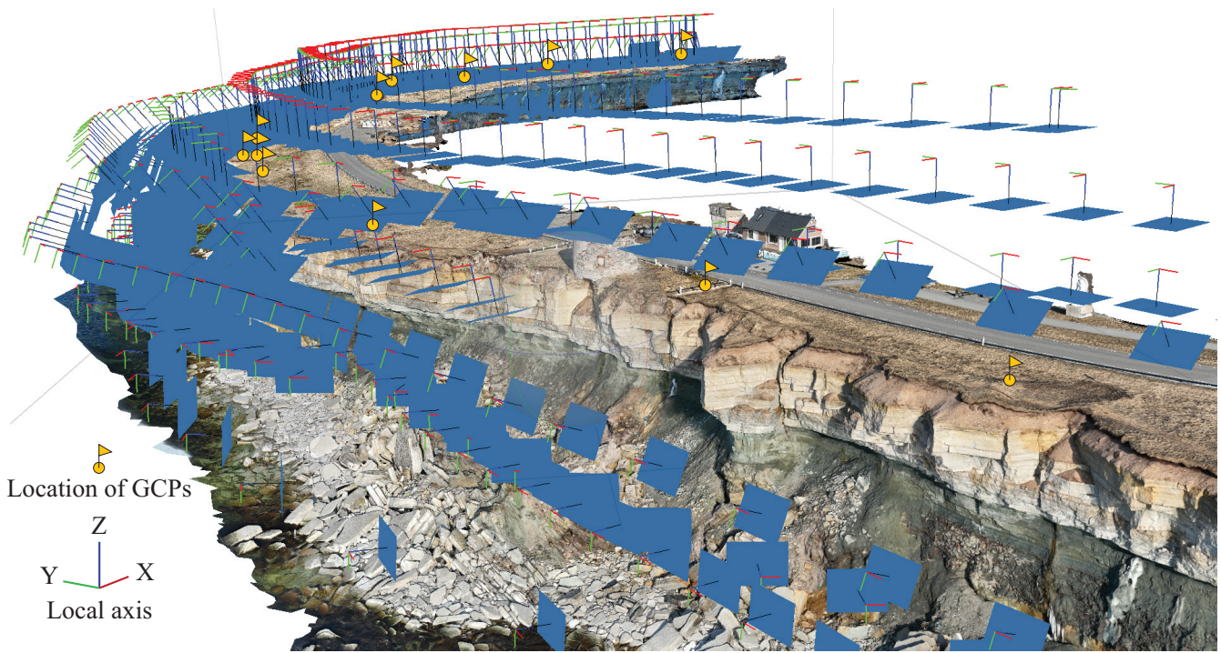
Fig. 4. Image coverage and ground control points (GCPs) in the March 2024 model.
