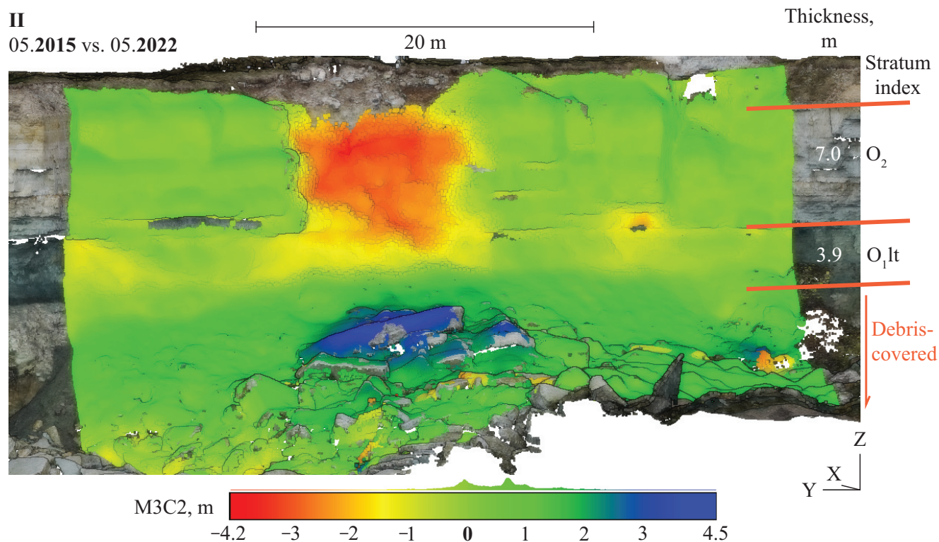
Fig. 11B. Section II – collapse of a limestone block next to the Pakri old lighthouse.
