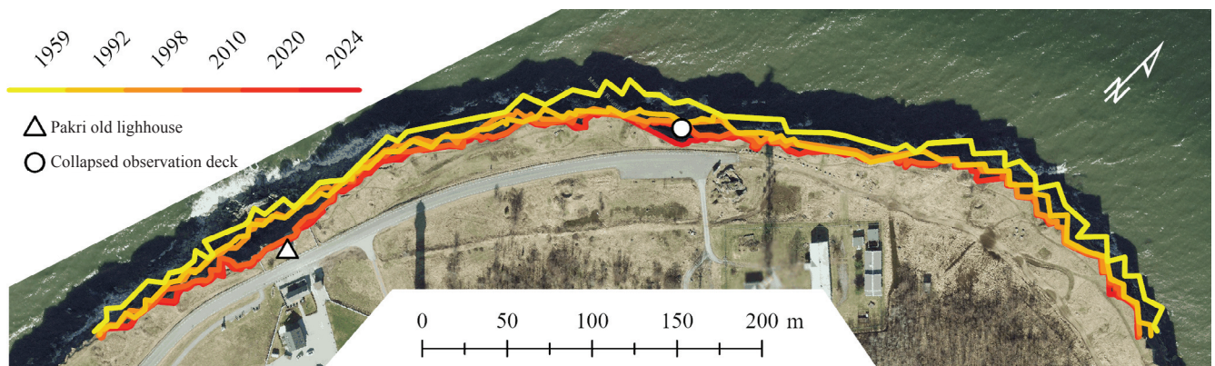
Fig. 10. Cliff edge retreat over 65 years.
