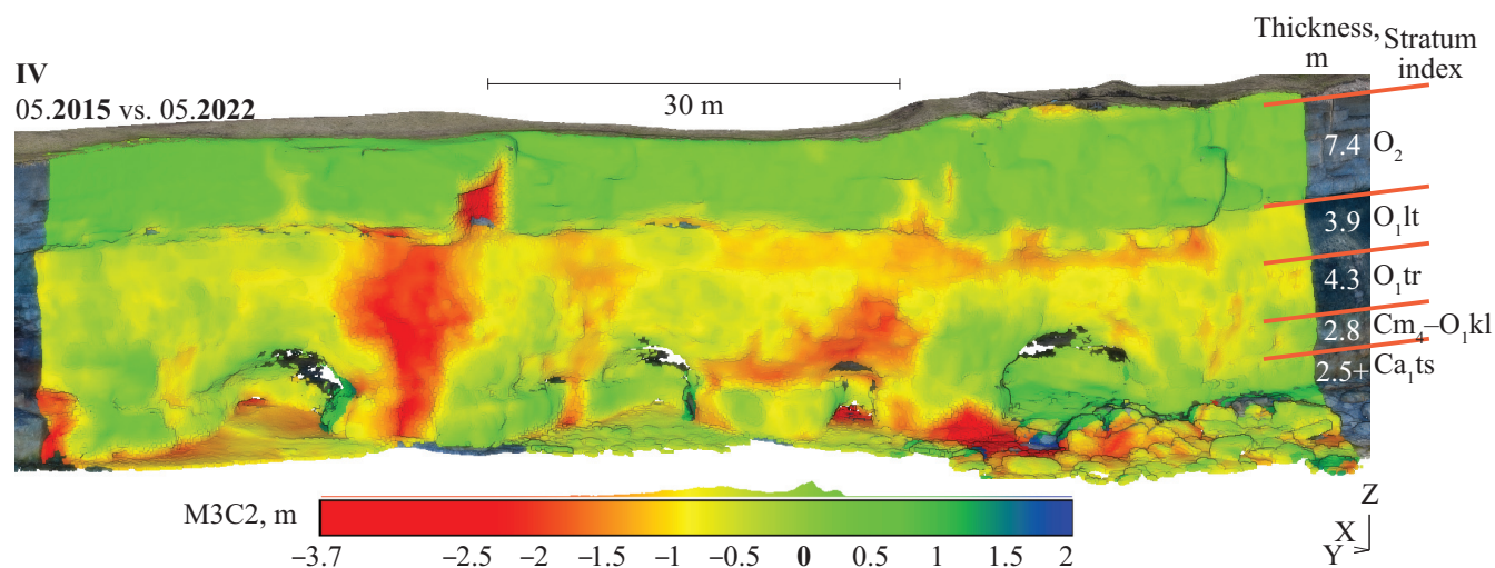
Fig. 11D. Section IV – coastal notches.
