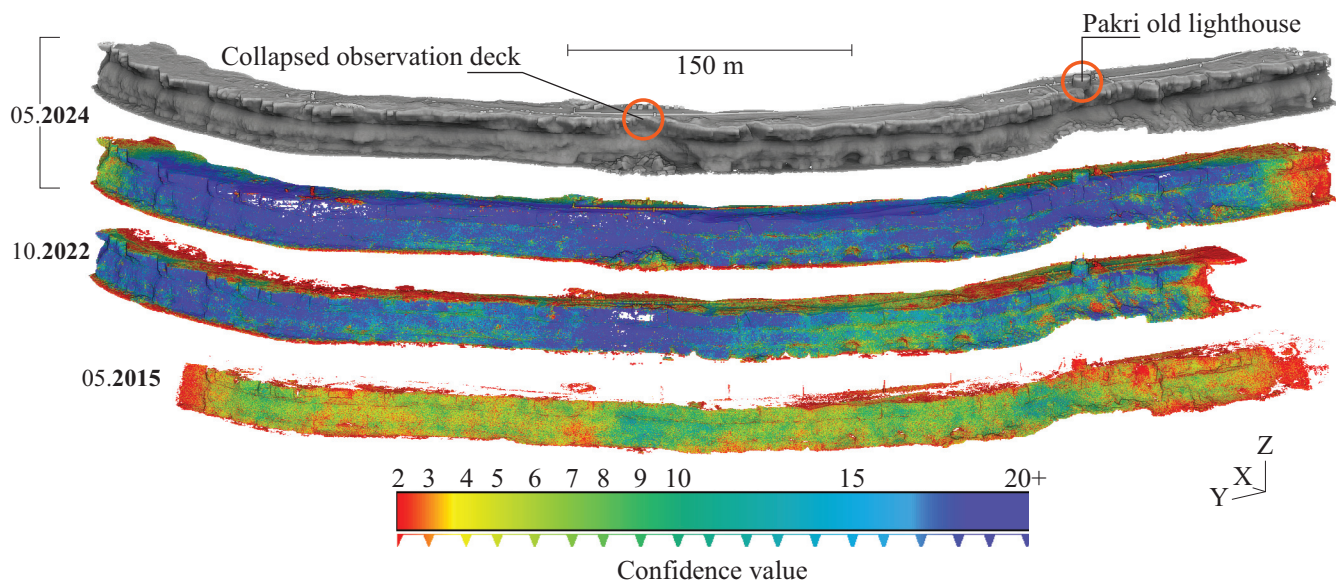
Fig. 5. Distribution of confidence values across point clouds. Values below 2 have been removed to improve accuracy.
