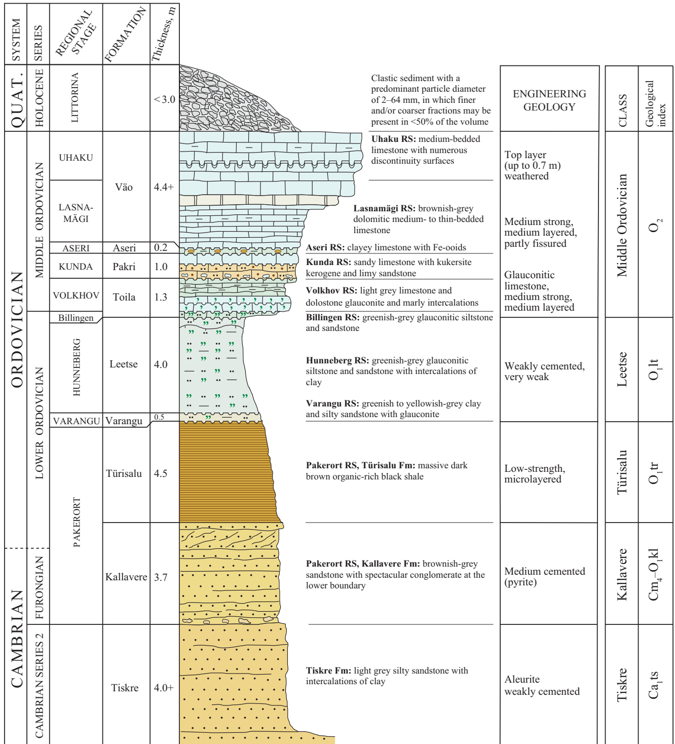
Fig. 2. Composite section of the Pakri Peninsula. Modified by Hints et al. (2024) after Mens and Puura (1996). The cross-section has been complemented with a description of the top layer, engineering geological data from the Estonian Geological Archive, and the classification used in the study. Abbreviations: QUAT. – Quaternary, RS – regional stage, Fm – formation.
