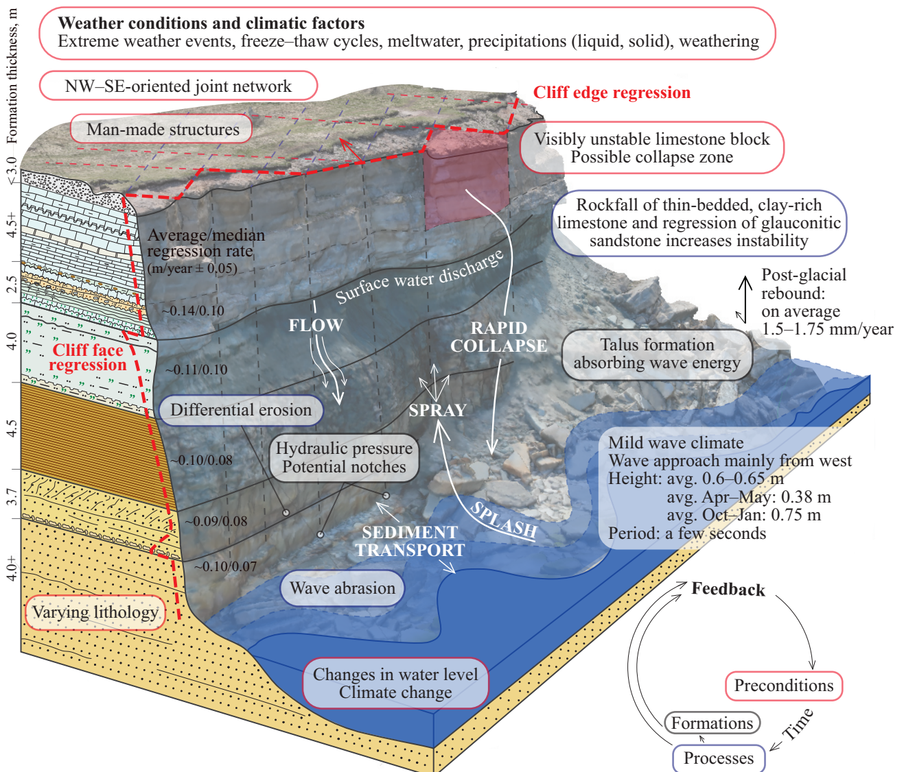
Fig. 12. Conceptual model of Pakri Cliff retreat. Average wave climate characteristics are adapted from Soomere and Räämet (2011), and the land uplift rate relative to the geoid is based on the NKG2016LU lev model (Suursaar and Kall 2018; Vestøl et al. 2019). A detailed overview of the relevant processes, controls, scales, and feedbacks is presented in Table 3.
