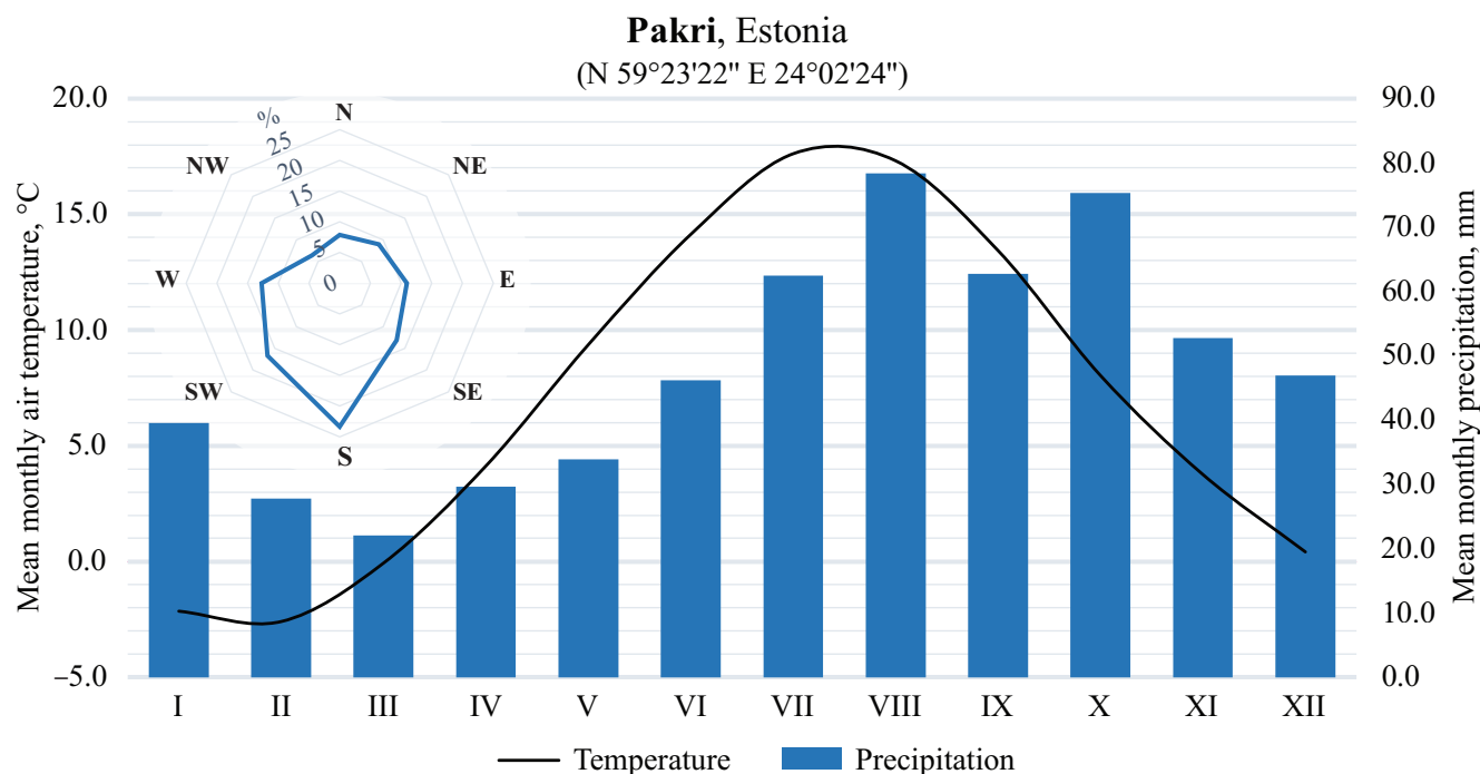
Fig. 3. Pakri climate diagram and wind rose based on measurements from the Pakri meteorological station. The figures are derived from hourly data collected over the past 20 years (January 2004 to December 2023). Precipitation measurements from November to March may differ from actual values, as the early data (2004–2009) were recorded using a device that was not operational during the winter season.
