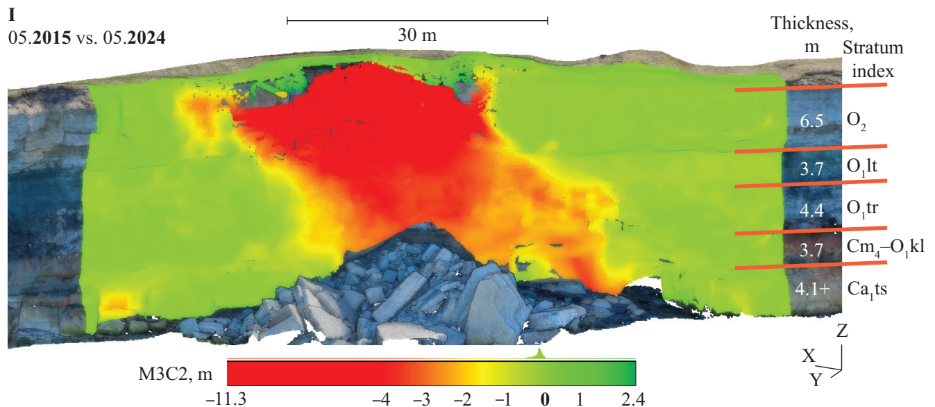
Fig. 11A. Section I – changes associated with the collapse of the Pakri observation deck.
