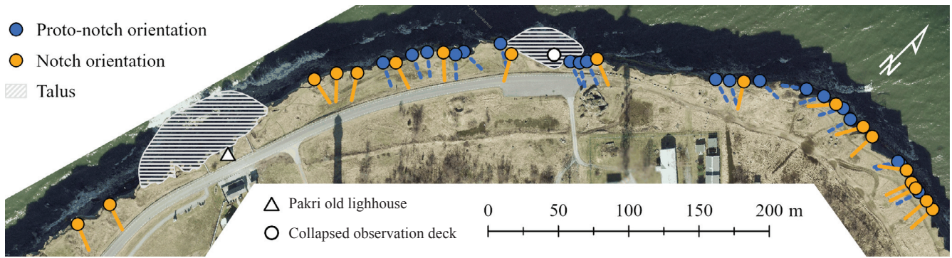
Fig. 9. Distribution and orientation of coastal notches and proto-notches.
