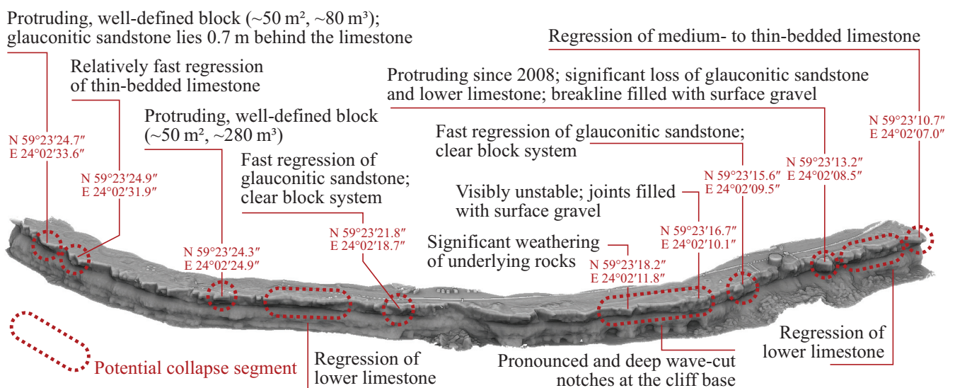
Fig. 13. Potential zones of cliff failure based on the authors' expert opinion.
