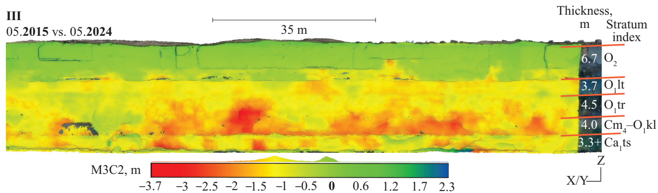
Fig. 11C. Section III – retreat of lower sandstone.
