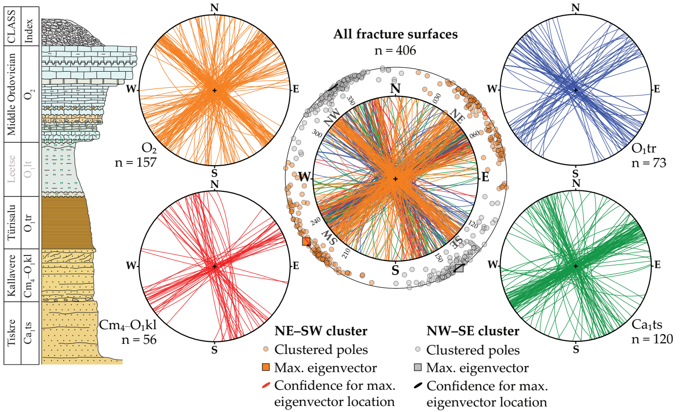
Fig. 7. Stereonets of mapped fracture surfaces, with clustered orientations plotted as poles. Projected on an equal-area lower hemisphere.
