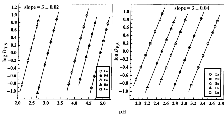
Fig. 1. Values of \log D_{T,S} and \log D_{P,S} vs. pH for the extraction of lanthanoid elements with HTTA-PAR and HP-PAR mixtures at [HTTA] = 3 \times 10^{-2} \text{ mol/dm}^3 , [HP] = 3 \times 10^{-2} \text{ mol/dm}^3 , and [PAR] = 4.86 \times 10^{-3} \text{ mol/dm}^3 .
