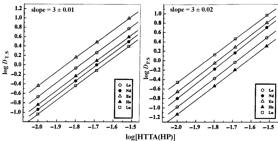
Fig. 2. Values of \log D_{T,S} and \log D_{P,S} vs. \log[HTTA, HP] for the extraction of lanthanoid elements with HTTA-PAR and HP-PAR mixtures at [PAR] = 4.86 \times 10^{-3} \text{ mol/dm}^3 . HTTA-PAR: La, pH = 5.15; Nd, pH = 4.60; Eu, pH = 4.0; Ho, pH = 3.25; Lu, pH = 2.55. HP-PAR: La, pH = 3.60; Nd, pH = 3.30; Eu, pH = 3.00; Ho, pH = 2.60; Lu, pH = 2.50.
