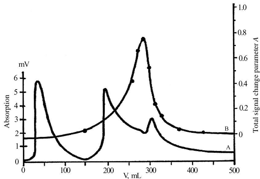
Fig. 2. Ion exchange chromatography of PSAO-containing extract on TEAE cellulose, elution with 0.1 M KCl in phosphate buffer (pH 7.0). The protein concentration was determined spectrophotometrically as absorption at \lambda = 280 nm (A). Amine oxidase (PSAO) activity was determined electrochemically by 0.12 mM cadaverine (B).
