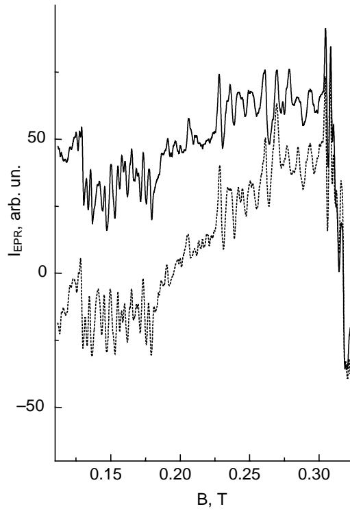
Fig. 3. EPR spectra of Mn^{2+} in low-symmetry field of Li_2B_4O_7:Mn,Si . The spectra show no basic difference between light-sensitive (...) and light-insensitive (-) samples.
