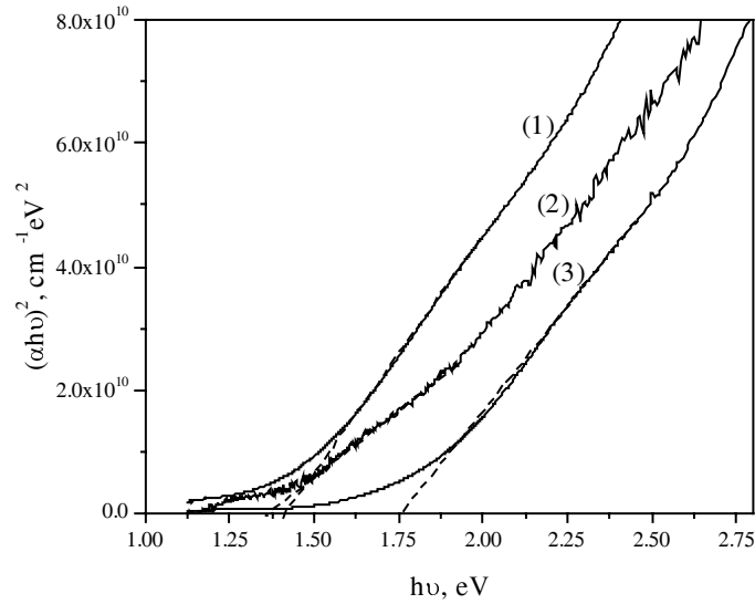
Fig. 4. The plot of (\alpha h\nu)^2 against the photon energy h\nu for the CIS thin films. (1) deposited onto In(O,S) and annealed in H_2 for about 30 min, (2) as-deposited, (3) deposited onto ITO and annealed in H_2S for about 30 min.
