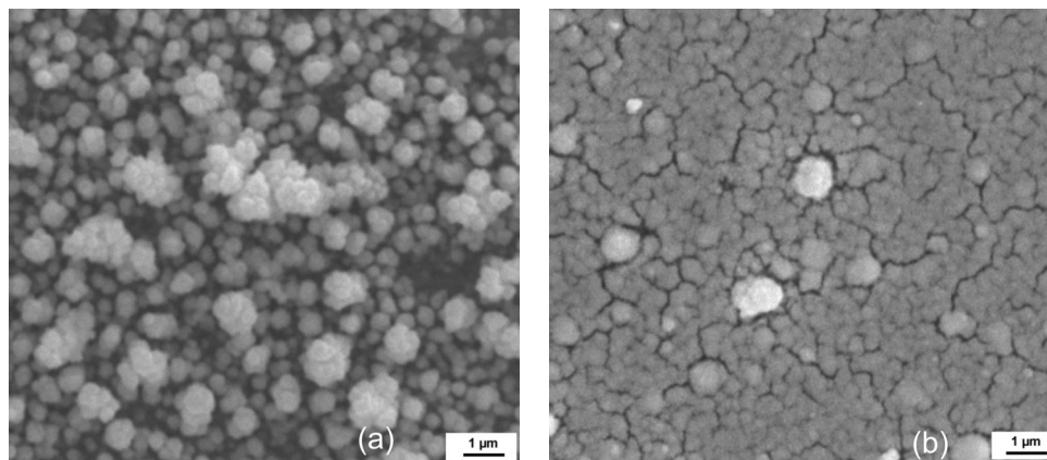
Fig. 1. Scanning electron micrographs of CIS thin films: (a) as-electrodeposited, (b) annealed at 450^\circ\text{C} in \text{H}_2\text{S} for 30 min.
