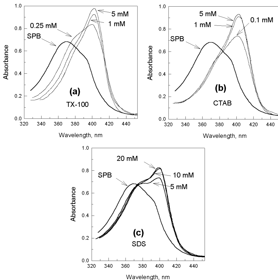
Fig. 4. Absorption spectra of the non-illuminated HPD ( 16.7 \mu\text{M} ) in 0.1 \text{ M} SPB of pH 7.4 ( 20^\circ\text{C} ) at different concentrations of: (a) Triton X-100 (TX-100), (b) cetyltrimethylammonium bromide (CTAB), and (c) sodium dodecyl sulphate (SDS) (sample light path, 0.5 \text{ cm} ).
