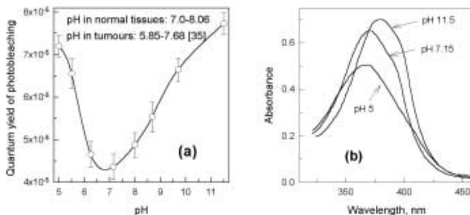
Fig. 2. Quantum yields of HPD (16.7 \mu M) photobleaching (a) and absorption spectra of the non-illuminated HPD (b) in aqueous solutions (20 °C) at different pH values. The experiments were performed in the buffer prepared by mixing 40 mM solutions of acetic, boric, and phosphoric acids (its pH was regulated by addition of 0.2 M NaOH). Bars are standard errors.
