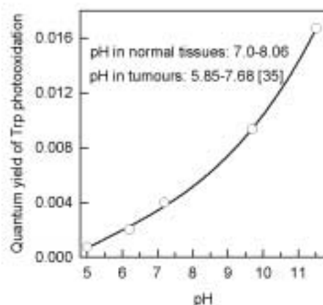
Fig. 3. Quantum yields of HPD (16.7 \mu M) photosensitized oxidation of 0.2 mM tryptophan in aqueous solutions of various acidity (at 20 °C). The buffer was the same as in Fig. 2.
