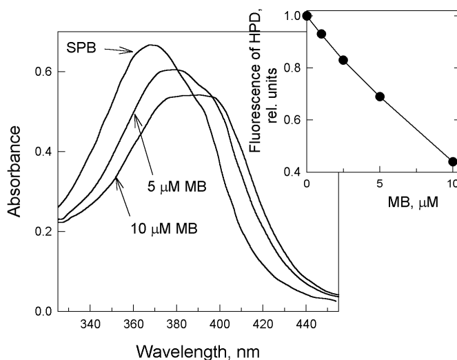
Fig. 5. Absorption spectra of the non-illuminated HPD (16.7 \mu\text{M} ) in 0.1 M SPB of pH 7.4 (20 ^{\circ}\text{C} ) at different concentrations of methylene blue (MB) (sample light path, 0.5 cm). Inset: fluorescence intensities of HPD solutions at 617 nm ( \lambda_{\text{ex}} = 400 nm) under the same conditions.
