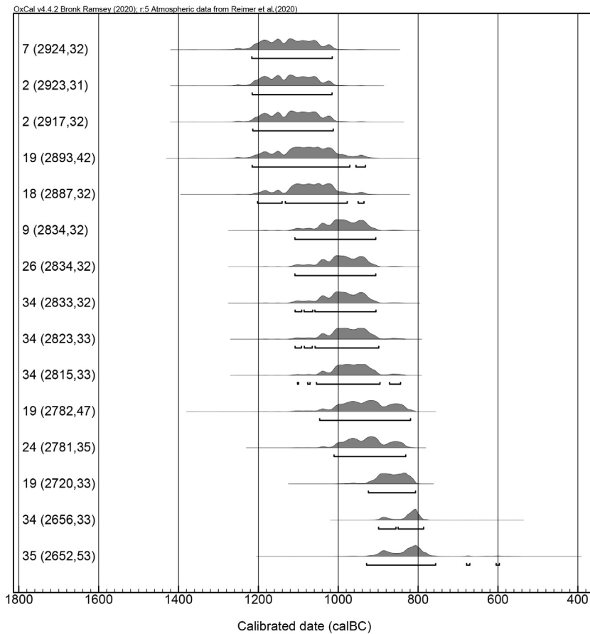
Fig. 2. AMS dates of the human bones from the stone-cist graves at Jöelähtme, corrected to calendar ages by OxCal v4.4.2 with IntCal20 calibration curve (Bronk Ramsey 2009; Reimer et al. 2020).
