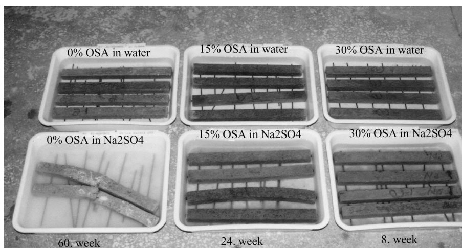
Fig. 1. Cure of mortar bars in water and sulphate solution [13].
