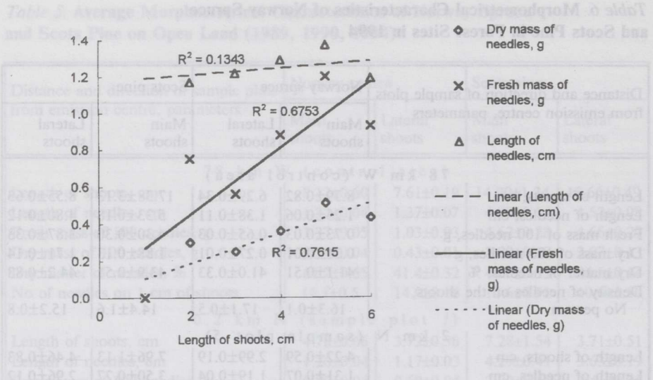
Fig. 3. Relationship between the length of shoots and needle development of Norway spruce. Regression trendlines and R-squared values were calculated using MS EXCEL 5.0
