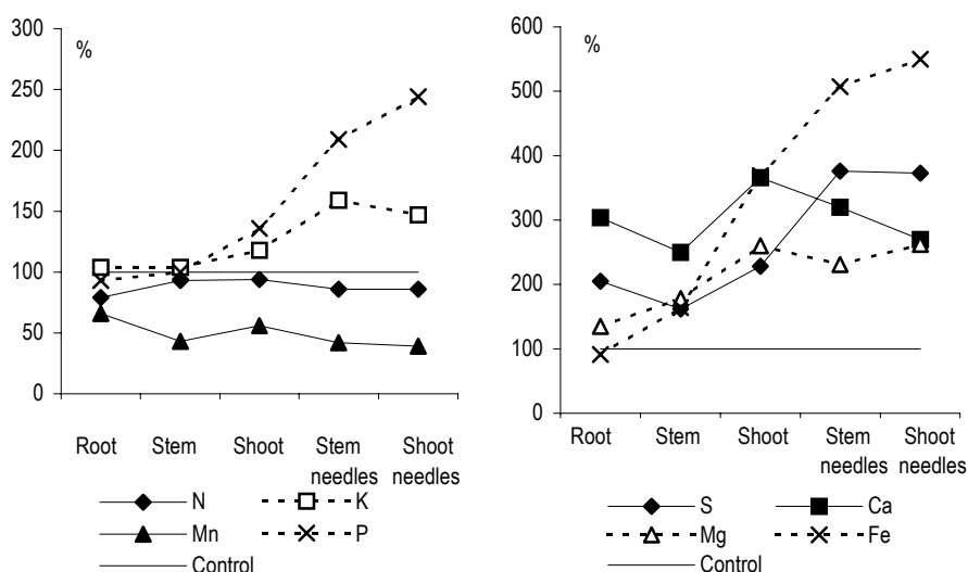
Fig. 2. Content of mineral elements in different components of Picea mariana in the area influenced by cement plant as percentage of control (100 %)
