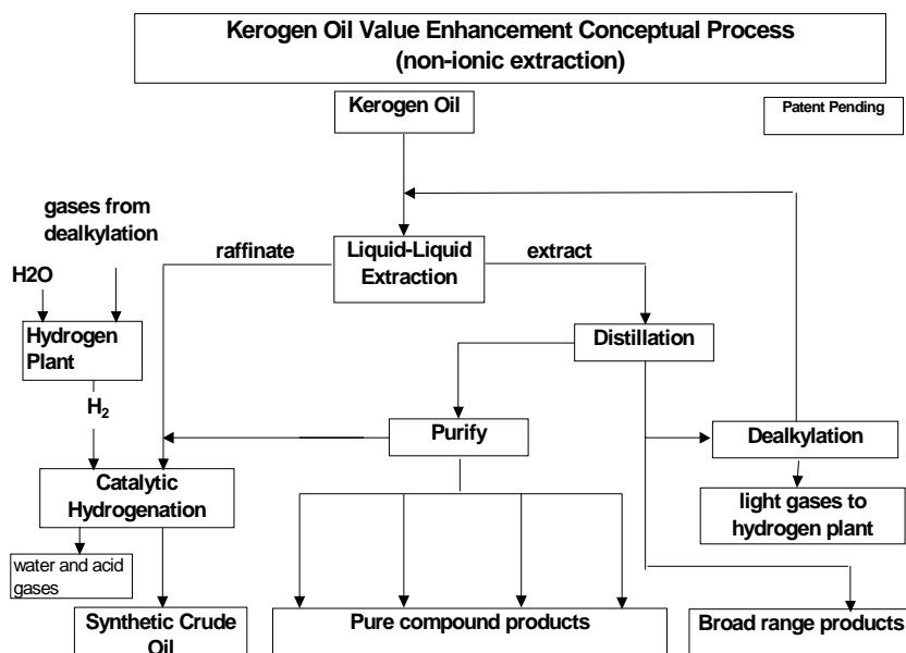
Fig. 1. Principal scheme of value enhancement process for treatment of kerogen oil based on separation by liquid-liquid extraction
