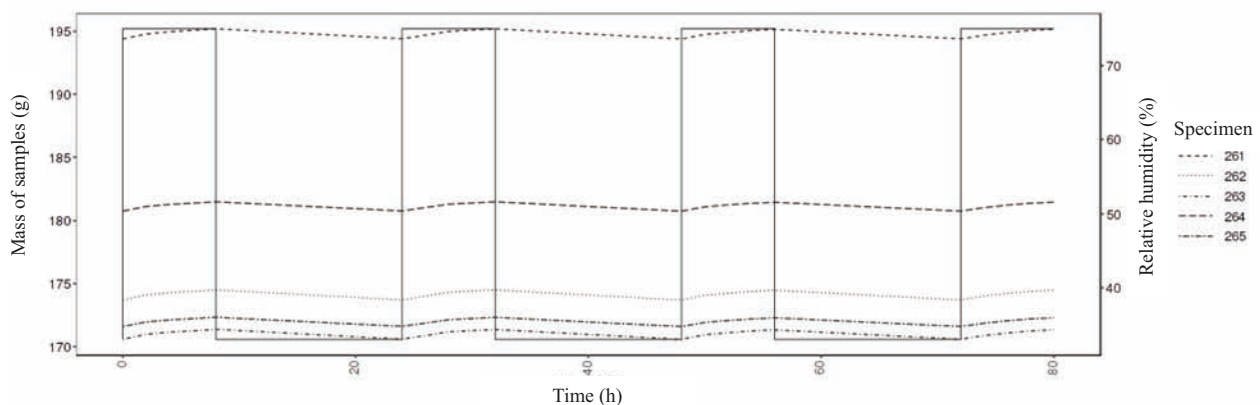
Fig. 2. The whole mass (g) of five samples (plaster group 5) in the cycles of Nordtest. The change in moisture cycles (RH 33% and RH 75%) in the climate chamber is portrayed by a continuous line.
