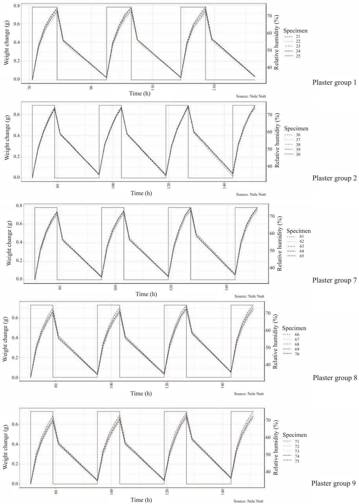
Fig. 3. Changes in specimens' weight (only weight change) in the final cycles (plaster groups 1, 2, 7, 8 and 9) of Nordtest. The change in moisture cycles (RH 33% and RH 75%) in the climate chamber is portrayed by a continuous line.
