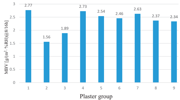
Fig. 4. MBV of plaster groups.
